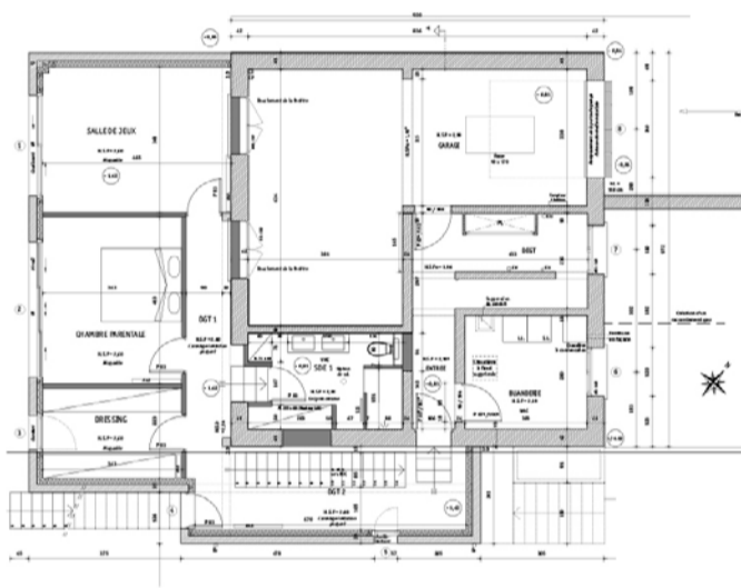
Rez-de-jardin (extension)
